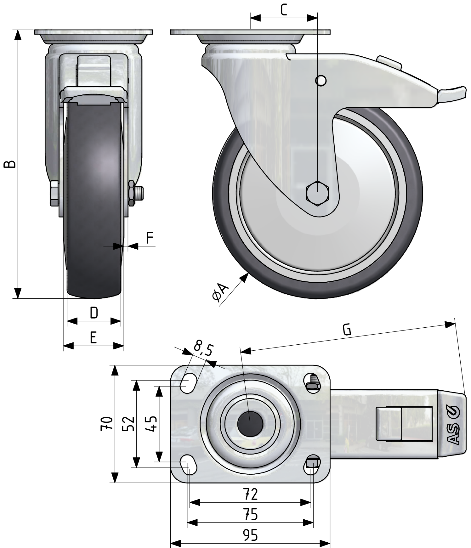
Massblatt NGSF Platte 95x70
